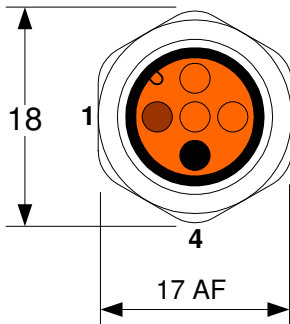
Face View 4 Pole 2 wire
